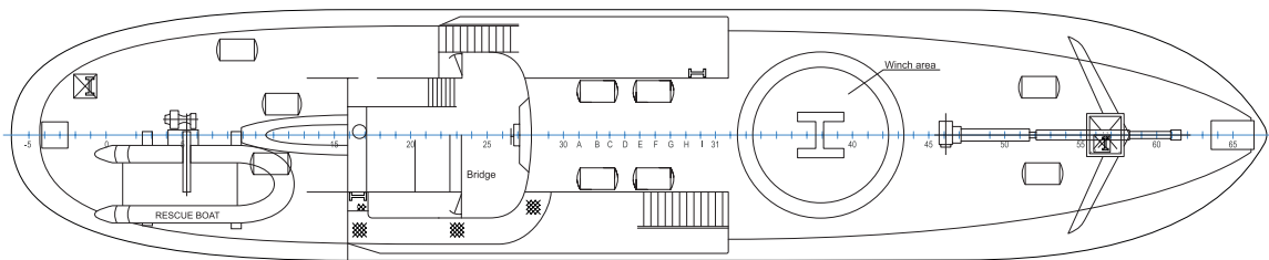
SHELTER DECK
